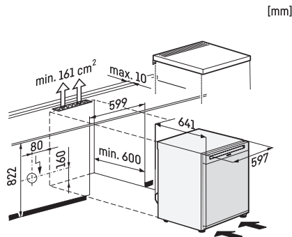
K4003D ws, K4002D ws, installation sketch
